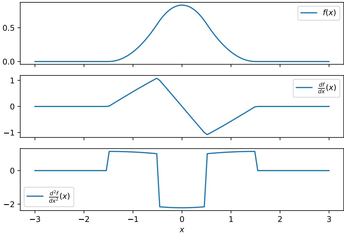
EM basis function and its derivatives for M = 5 , \alpha = 0.5
